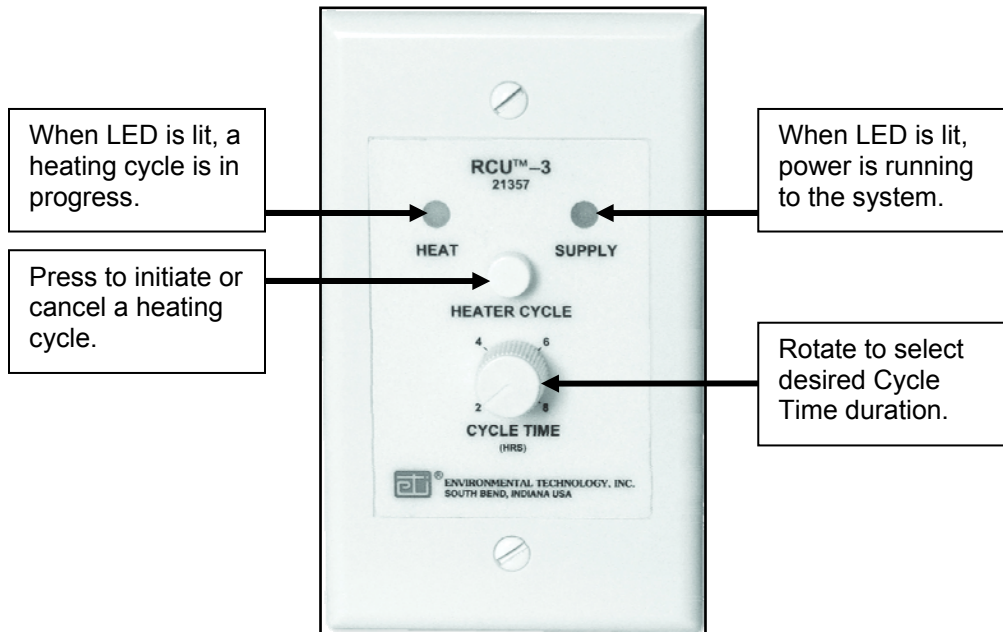
Figure 7. REMOTE CONTROL UNIT RCU-3.
