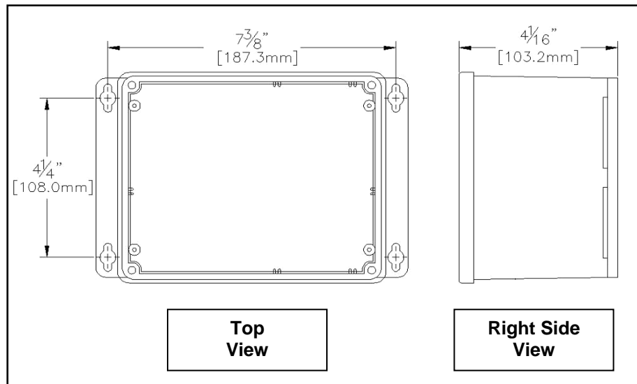
Figure 1. PD Pro MOUNTING HOLE FOOTPRINT.
