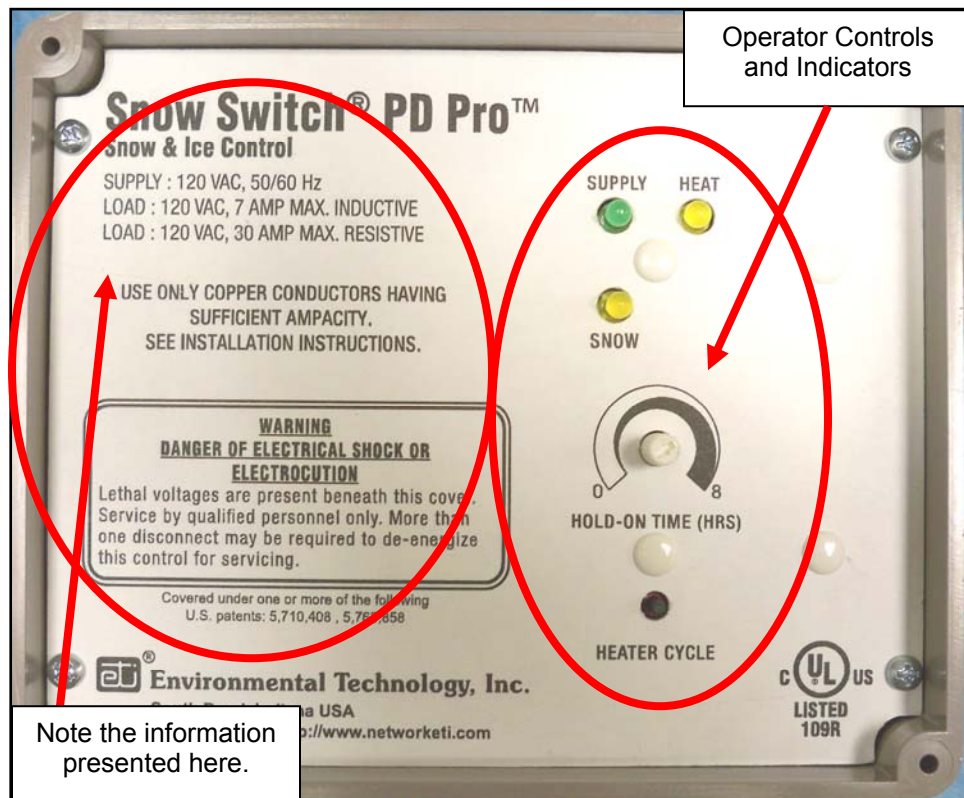
Figure 5. THE PD Pro FRONT PANEL.
